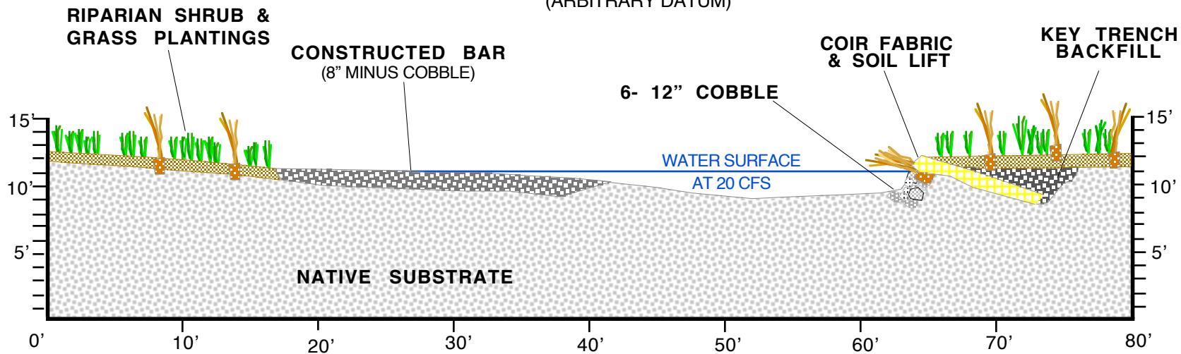
RUN OR POOL TAIL OUT & SINGLE COIR FABRIC LIFT X-SECTION
