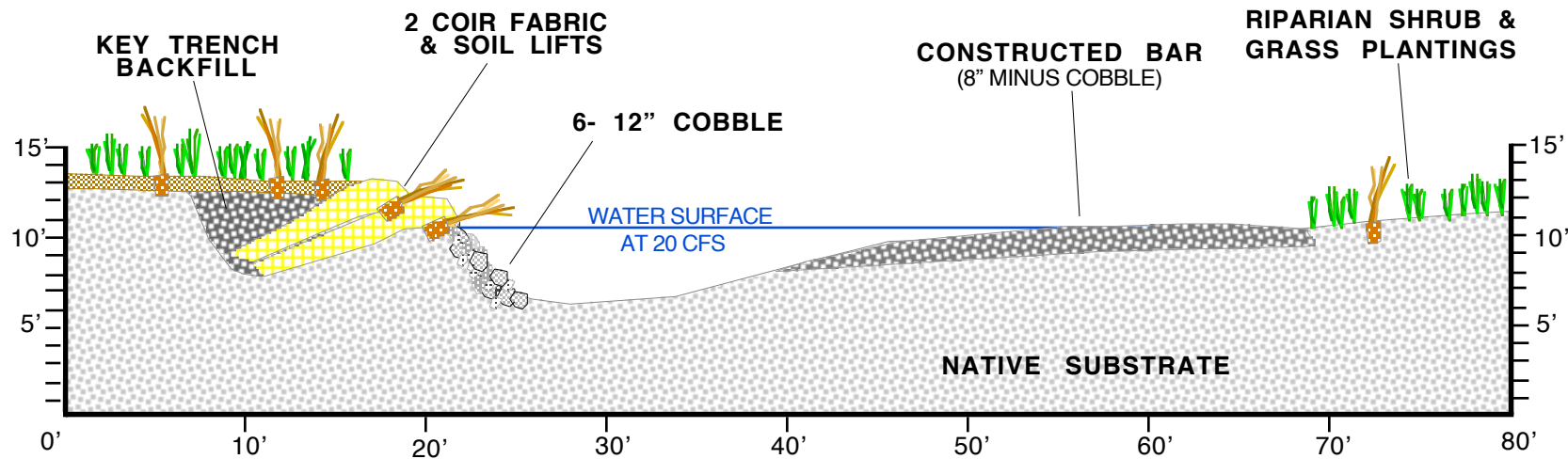
POOL & TWO COIR FABRIC LIFTS X-SECTION
